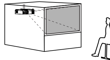
INSTALLATION: REAR/CEILING
